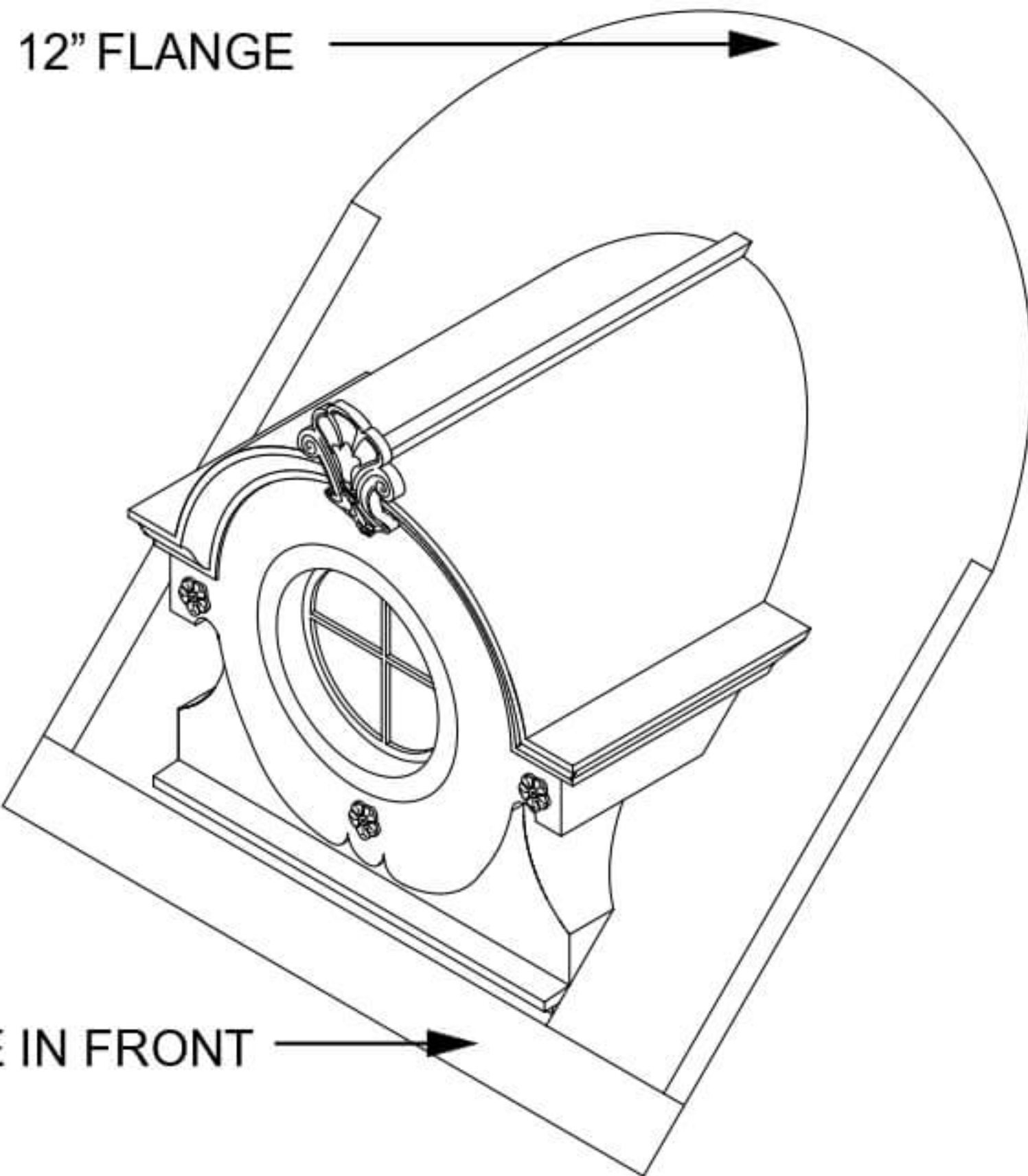
Isometric View Under Roofing:
